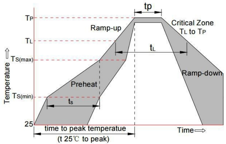
FIG.2: Reflow condition
