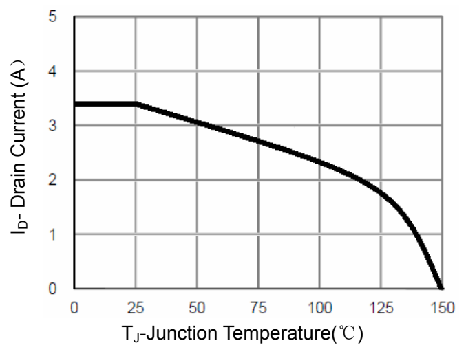
Figure 4 Drain Current
